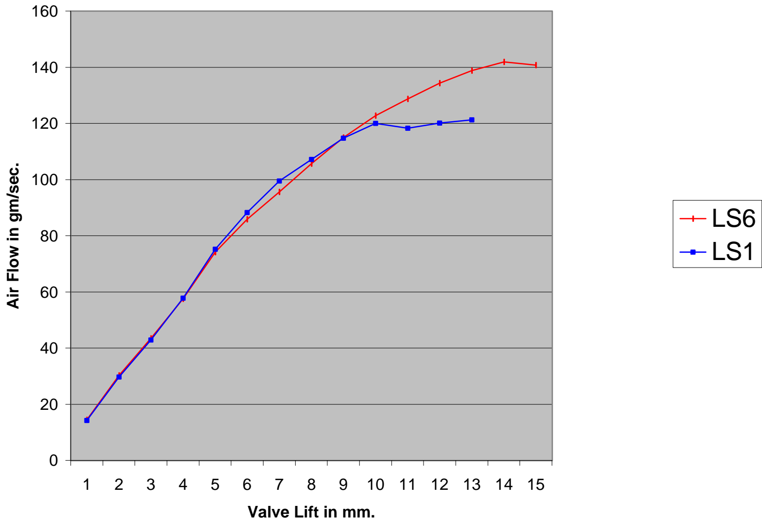
Intake Air Flow LS1 vs LS6
